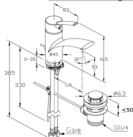
Dimensional drawing
