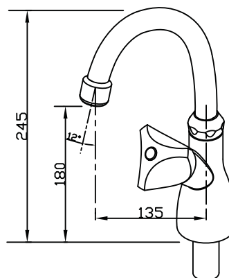
Dimensional Drawing
