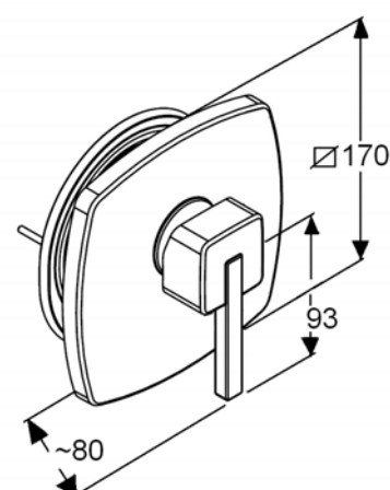
Dimensional drawing
