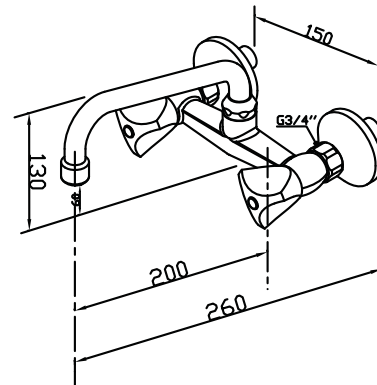
Dimensional Drawing
