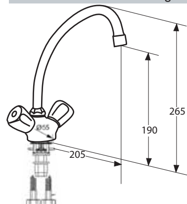
Dimensional Drawing
