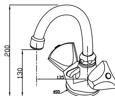
Dimensional Drawing
