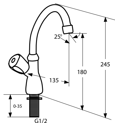
Dimensional Drawing
