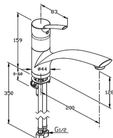
Dimensional drawing
