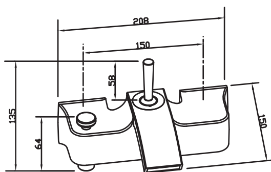
Dimensional Drawing
